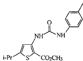
35 5-Isopropyl-3-(3-p-tolyl-ureido)-thiophene-2-carboxylic acid methyl ester
